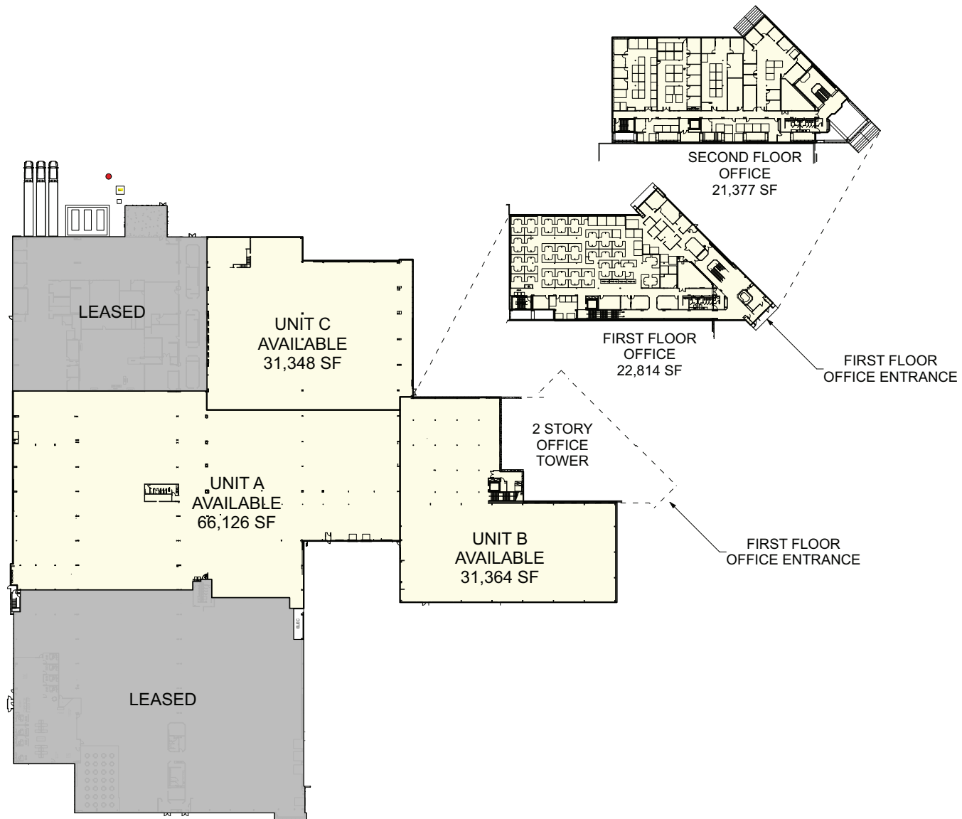
3 MULTI TENANT FLOORPLAN Scale: 1" = 40'-0"
